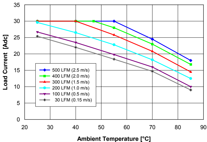
Fig. 11: Available load current vs. ambient air temperature and airflow rates for converter mounted vertically with V_{in} = 54 V, air flowing from pin 3 to pin 1 and maximum FET temperature \leq 105^{\circ}\text{C} .
