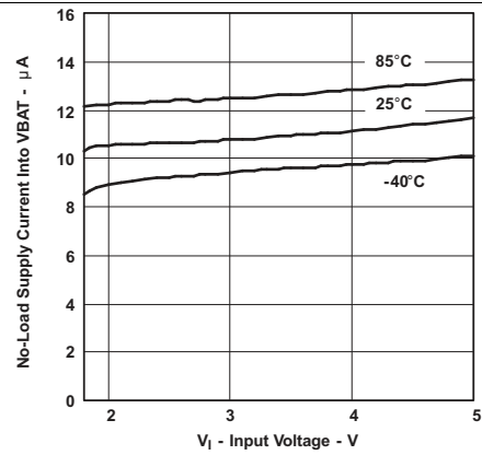
Figure 10. TPS61092 No-Load Supply Current Into VBAT Voltage
