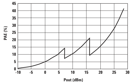
Figure 29. PAE (3-mode control).
