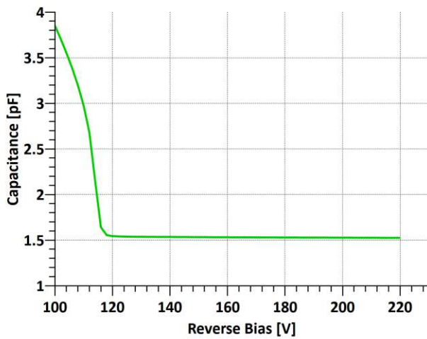
Figure 7: Typical Capacitance
