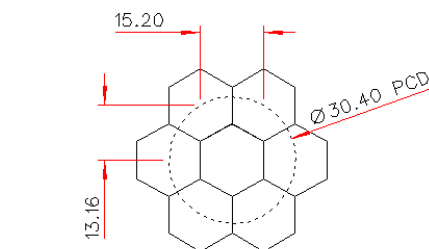
NESTED COMPONENTS ON 30.4MM PCD
