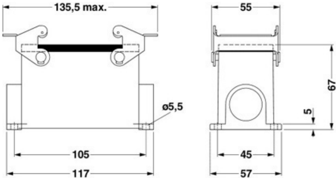
Dimensioned drawing
