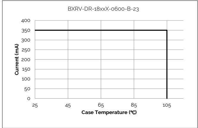
Figure 12: Derating Curve
