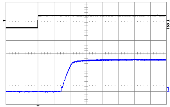
Figure 17. Turn-on transient at full rated load current (resistive) with no out-put capacitor at V_{in} = 48\text{ V} , triggered via ON/OFF pin. Top trace: ON/OFF signal (5 V/div.). Bottom trace: output voltage (2 V/div.) Time scale: 1 ms/div.
