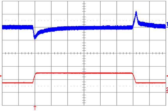
Figure 19. Output voltage response to load current step-change (3.75 A – 7.5 A – 3.75 A) at V_{in} = 48 V. Top trace: output voltage (100 mV/div). Bottom trace: load current (5 A/div). Current slew rate: 0.1 A/ \mu s. C_o = 1 \mu F ceramic. Time scale: 0.2 ms/div.
