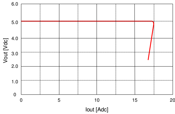
Figure 25. Output voltage vs. load current showing current limit point and converter shutdown point. Input voltage has almost no effect on current limit characteristic.
