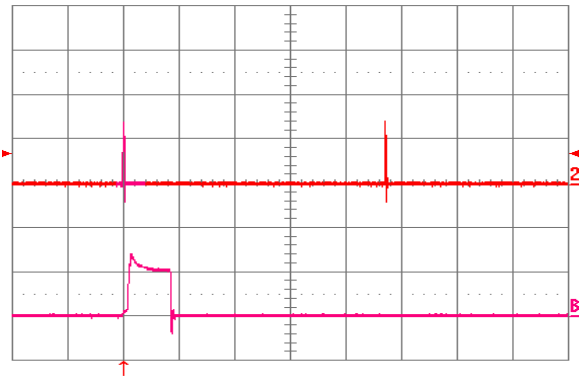
Figure 26. Load current (top trace, 20 A/div, 20 ms/div) into a 10 mΩ short circuit during restart, at Vin = 48 V. Bottom trace (20 A/div, 1 ms/div) is an expansion of the on-time portion of the top trace.
