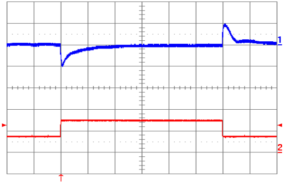
Figure 20. Output voltage response to load current step-change (3.75 A – 7.5 A – 3.75 A) at V_{in} = 48 V. Top trace: output voltage (100 mV/div). Bottom trace: load current (5 A/div). Current slew rate: 5 A/ \mu s. C_o = 450 \mu F tantalum + 1 \mu F ceramic. Time scale: 0.2 m
