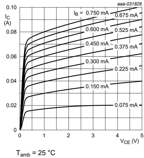
Fig. 17. NHDT114YU: Collector current as a function of collector-emitter voltage; typical values
