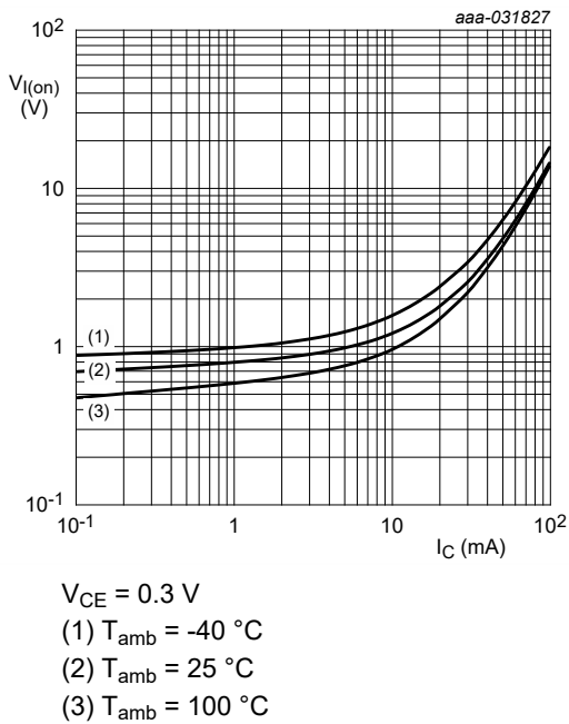
Fig. 18. NHDT114YU: On-state input voltage as a function of collector current; typical values
