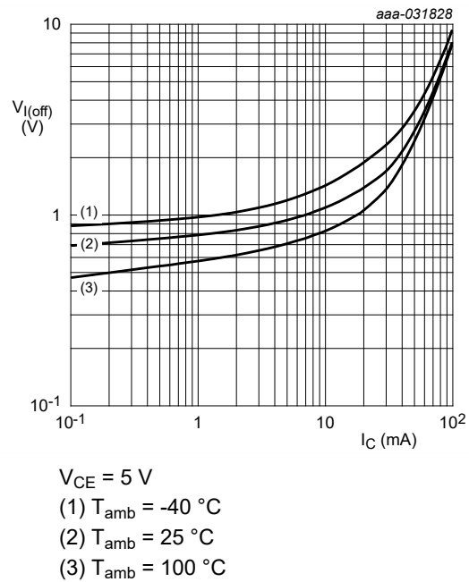
Fig. 19. NHDT114YU: Off-state input voltage as a function of collector current; typical values
