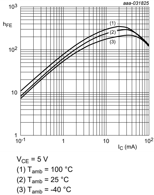
Fig. 16. NHDT114YU: DC current gain as a function of collector current; typical values
