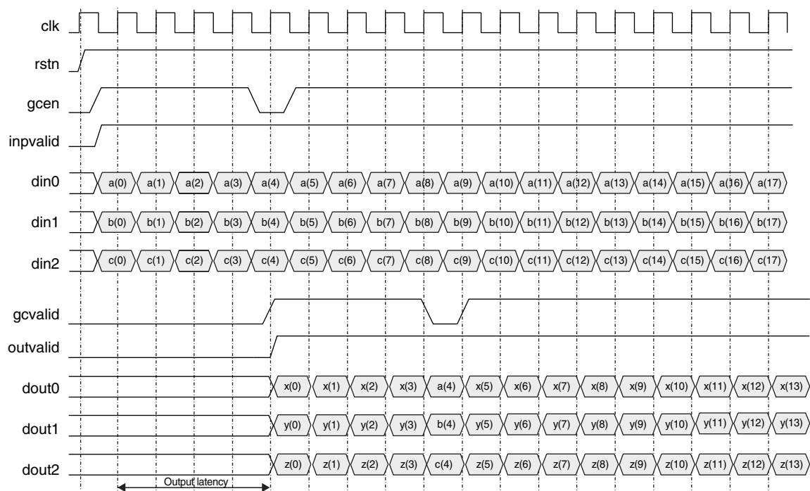
Figure 2-3. Parallel Architecture
