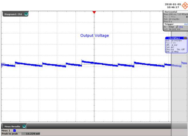
Figure 68 – Output Ripple. 180 VAC Input 5.1 V, 6.0 A Load. V_{OUT} , 20 mV / div., 10 ms / div.
