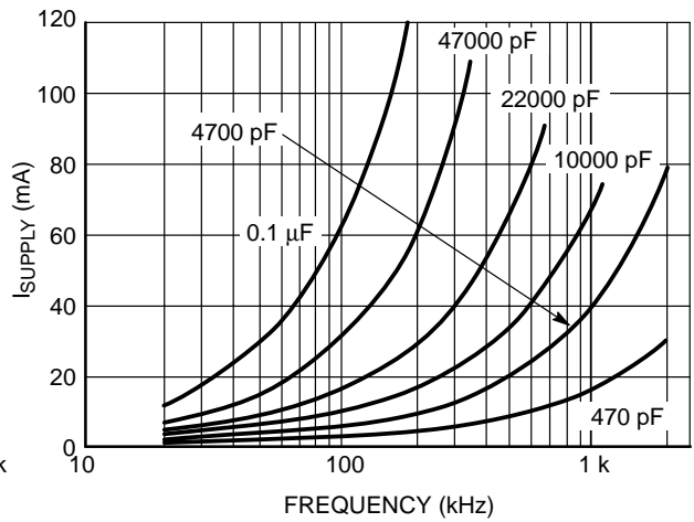
Figure 13. Supply Current vs. Frequency (V DD = 6 V)
