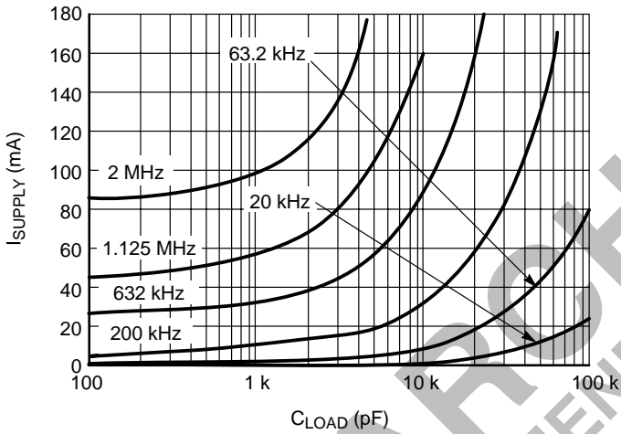
Figure 10. Supply Current vs. Capacitive Load (V DD = 12 V)
