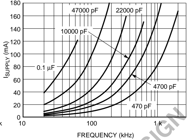
Figure 9. Supply Current vs. Frequency (V DD = 18 V)
