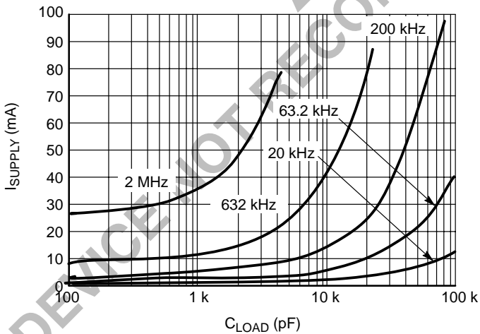
Figure 12. Supply Current vs. Capacitive Load (V DD = 6 V)
