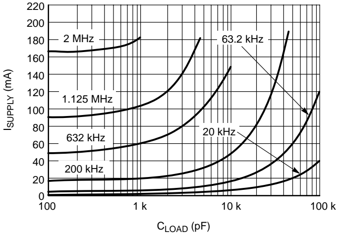
Figure 8. Supply Current vs. Capacitive Load (V DD = 18 V)
