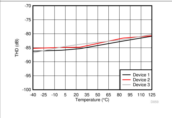
Figure 6-26. Total Harmonic Distortion vs Temperature
