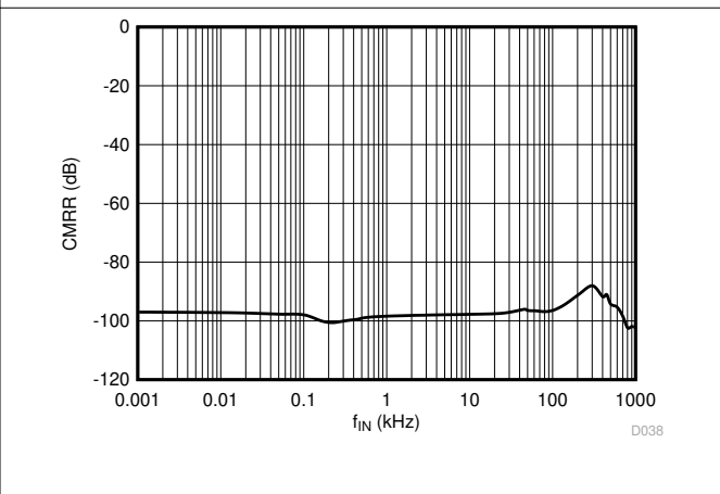
Figure 6-28. Common-Mode Rejection Ratio vs Input Frequency
