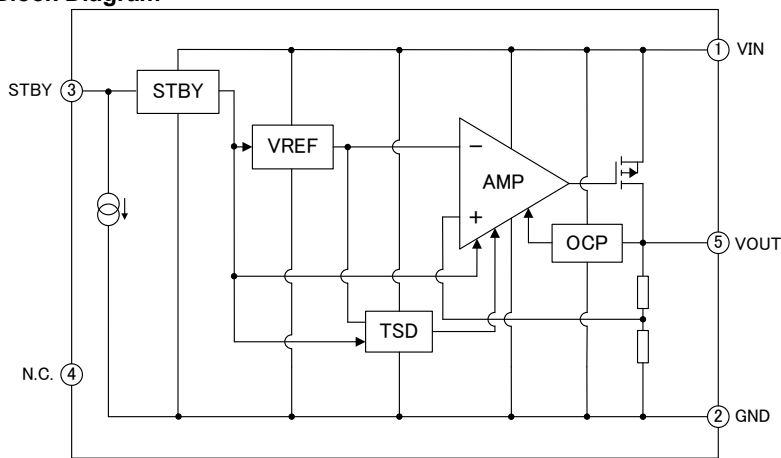
Figure 2. Block diagram
