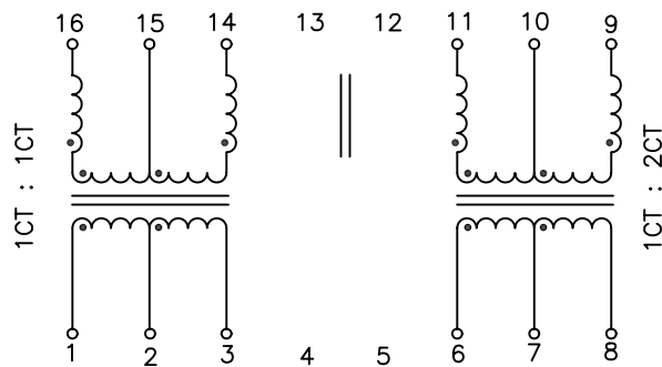
SCHEMATIC
