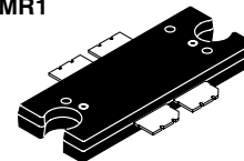
CASE 1484-03, STYLE 1 TO-272 WB-4 PLASTIC MRF6S9125MBR1
