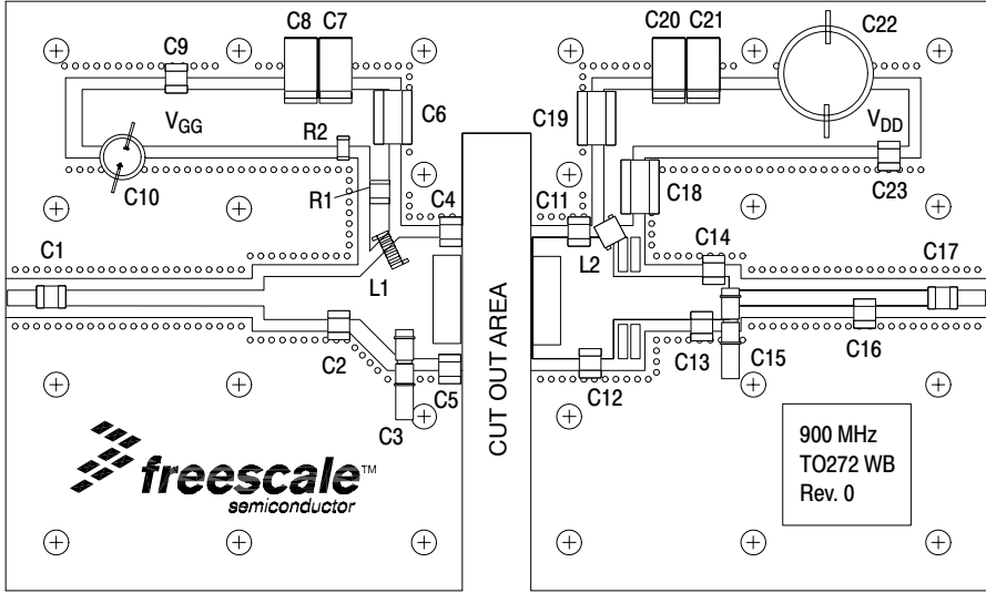
Figure 2. MRF6S9125MR1 (MBR1) Test Circuit Component Layout
