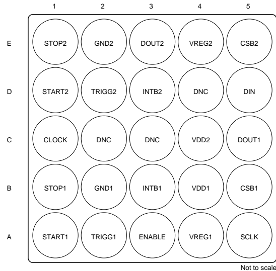
ZAX Package 25-Pin nFBGA Bottom View
