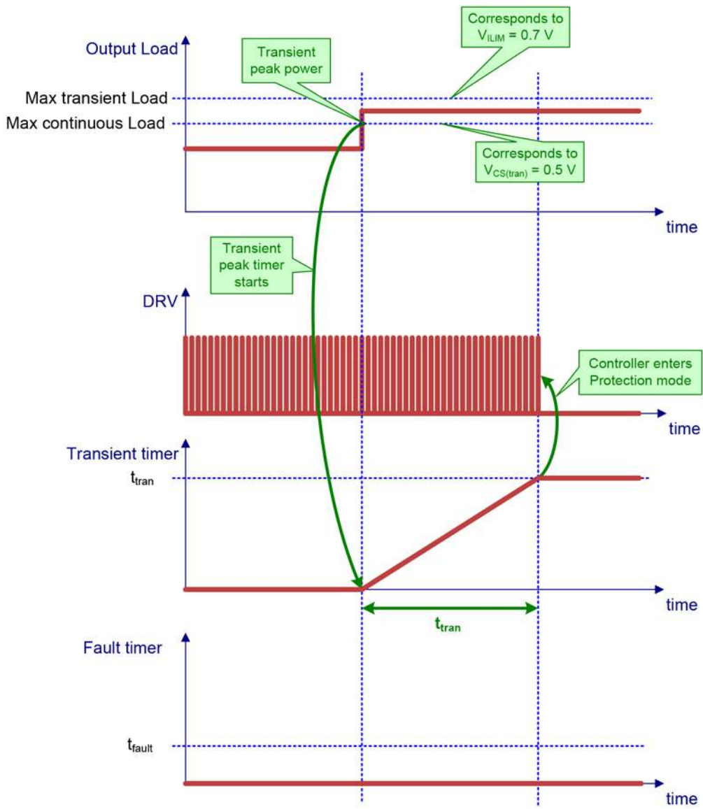
Figure 72. Too Long Transient Peak Power Delivery
