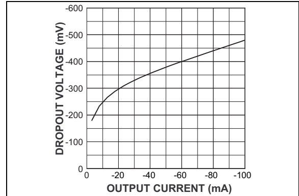
FIGURE 2-11: Dropout Voltage vs. Output Current.
