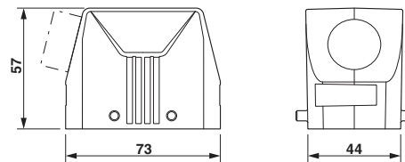
Dimensional drawing
