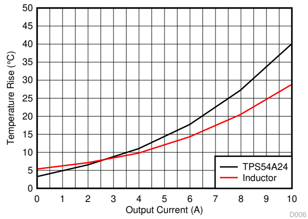
Figure 2-19. TPS54A24EVM-058 Thermal Performance
