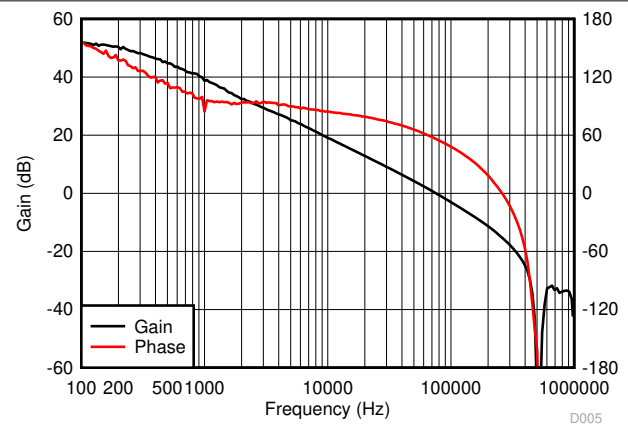
Figure 2-6. TPS54A24EVM-058 Loop Response
