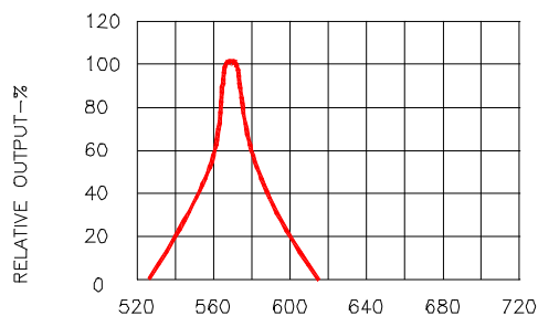
Fig.2 SPECTRAL RESPONSE
