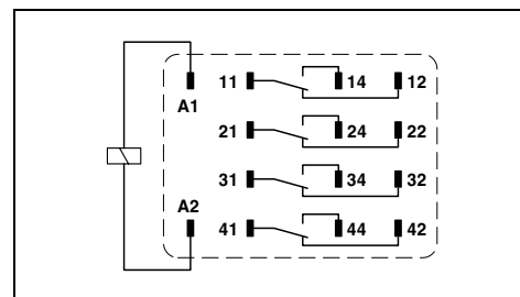
Industrial relay with four changeover contacts (non-polarized) with manual operation, 4 x 6 A, maximum
