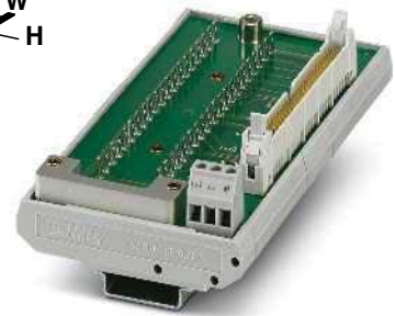
Converter for SIMATIC® S5-95U to 50-pos. IDC/FLK pin strip
