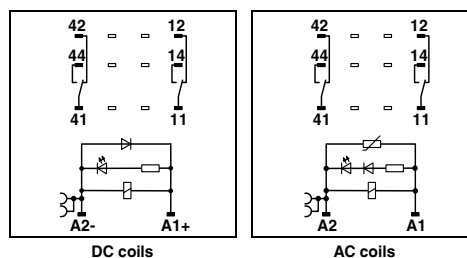
2-changeover-contact industrial relay module with Push-in connection and manual operation
