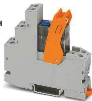
2-changeover-contact relay module with screw connection and manual operation
