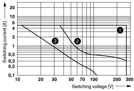
① AC, ohmic load ② DC, ohmic load ③ DC, L/R = 40 ms Interrupting rating
