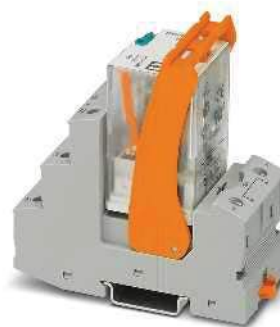
2-changeover-contact octal relay module with screw connection and manual operation
