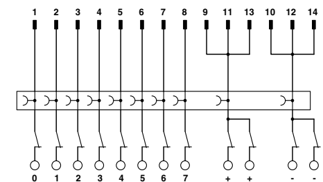
Connection scheme FLKM 14/KDS3-MT/PPA/PLC
