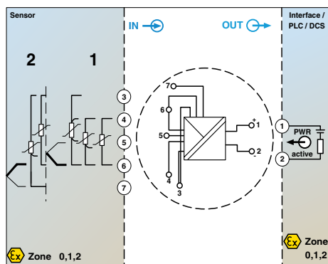
Loop-powered temperature head-mounted transducer
