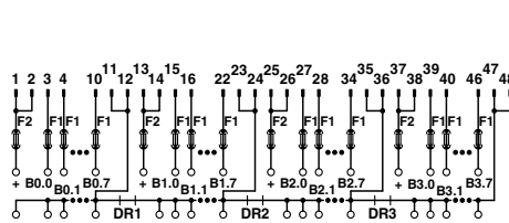
Connection scheme: FLKM 50/32M/SI/PLC
