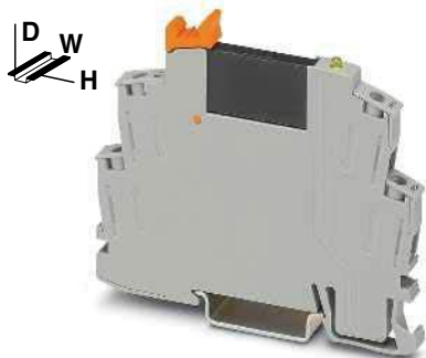
Solid-state relay module with screw connection, DC output max. 100 mA
