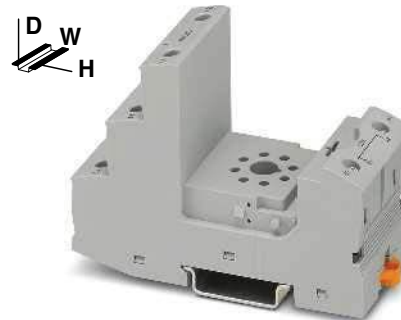
2-changeover-contact relay base with screw connection technology for octal relays
