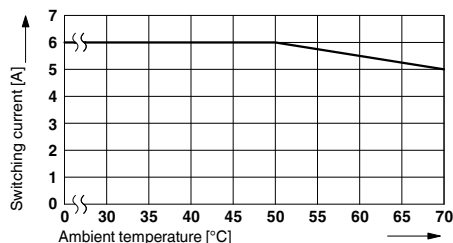
Derating curve for PLC-RSP...21/RW PLC-RSP...21AU/RW PLC-RSP...21-21/RW PLC-RSP...21-21AU/RW
