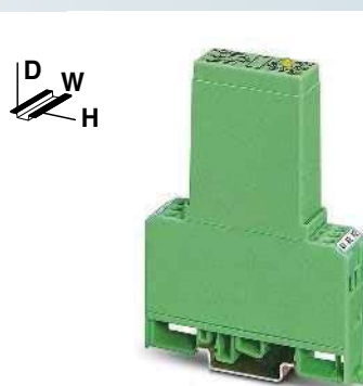
Solid-state power relay max. 2 A
