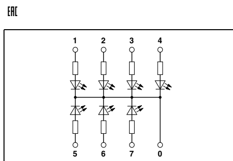
Light indicator module, with common return line
