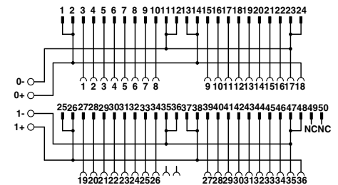
Connection scheme FLKM 50-PA-AB/1756/EXTC
