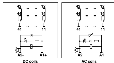
2-changeover-contact industrial relay module with screw connection and manual operation
