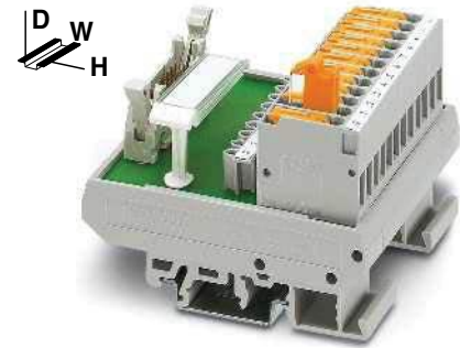
Passive termination board for 8 or 32 channels with knife disconnect terminal blocks
