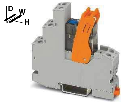
1-changeover-contact relay module with screw connection and manual operation
