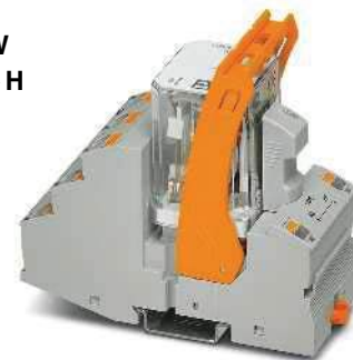
3-N/O-contact high-power relay module with Push-in connection
