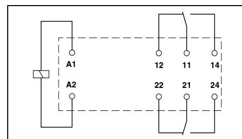
Relay with two changeover contacts with manual operation, 2 x 8 A, maximum
