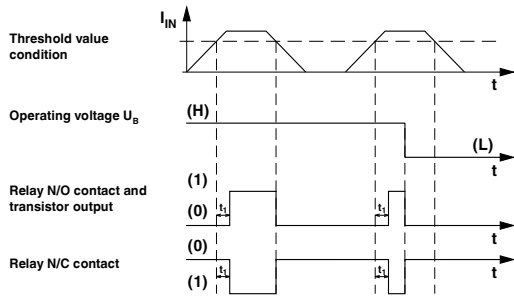
Function chart: switching behavior of relay and transistor output:
