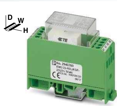
1 changeover contact, soldered-in relay
