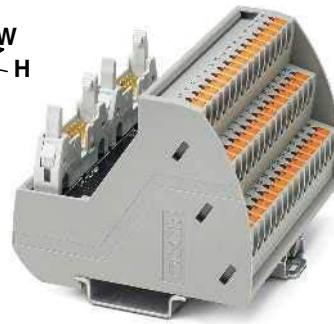
Passive termination board for SIMATIC® S7-1500 with separate potentials
