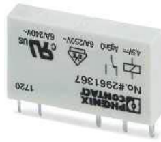
Relay with one changeover contact, max. 6 A
