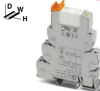
1-N/O-contact relay module with additional floating terminal point, 800 A peak, maximum
