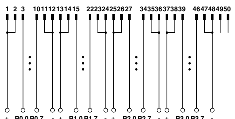
Connection scheme VIP-2/SC/FLK50/PLC
