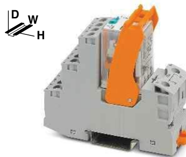
2-changeover-contact industrial relay module with screw connection and manual operation
