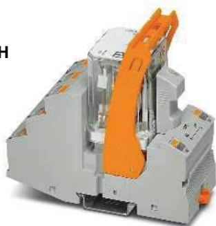
3-changeover-contact high-power relay module with Push-in connection
