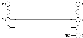
Connection scheme PLC-VT
