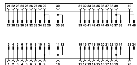
Connection scheme FLKM 50-PA/AN/S7-1500
