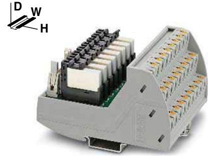
Digital input module with 8 channels for 120 V AC
