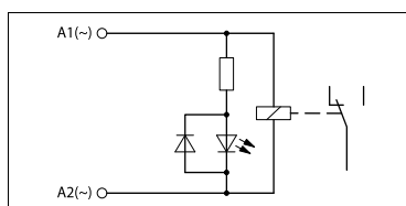
Basic structure of a relay with AC input
