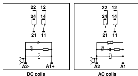
2-changeover-contact octal relay module with Push-in connection and manual operation
