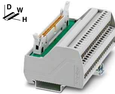
Passive interface module for input/output with screw connection
