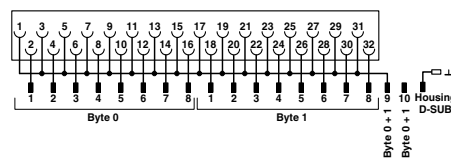
Connection scheme FLKM-PA-2D15/HW/DI/C300
