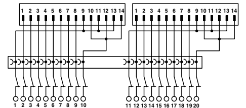
Connection scheme FLKM-2FLK14/KDS3-MT/PPA/S7
