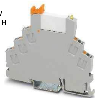
1-changeover-contact relay module with Push-in connection
