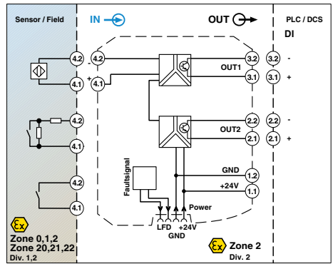
NAMUR signal conditioner: 2 signal outputs: transistor (passive)
