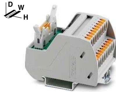
Passive interface module with Push-in connection
