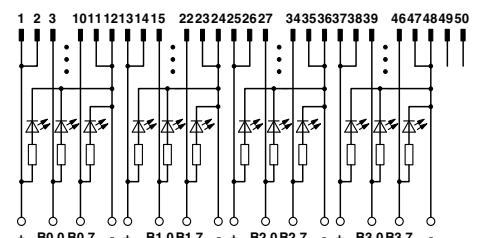
Connection scheme VIP-2/SC/FLK50/LED/PLC
