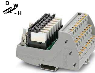
Digital input module with 8 channels for 24 V DC
