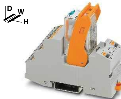
2-changeover-contact industrial relay module with Push-in connection and manual operation
