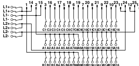
FLKM-D25 SUB/B/KDS3-MT/TU830 connection scheme
