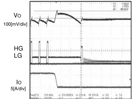
Fig.6 Transitional response ( I_o=5 \rightarrow 0A ) (SLLM™)
