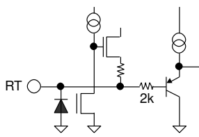
Figure 52. RT
