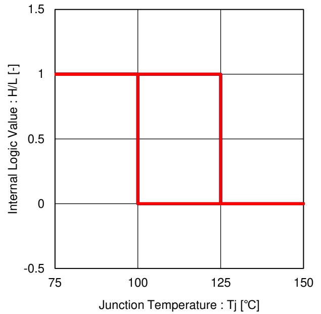
Figure 43 Thermal Shutdown
