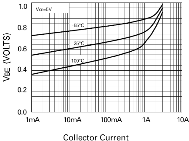
V_{BE(ON)} vs I_C
