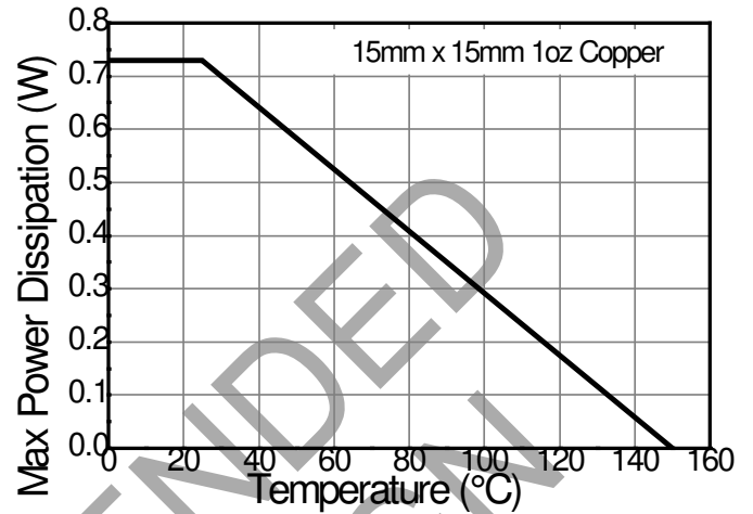
Derating Curve
