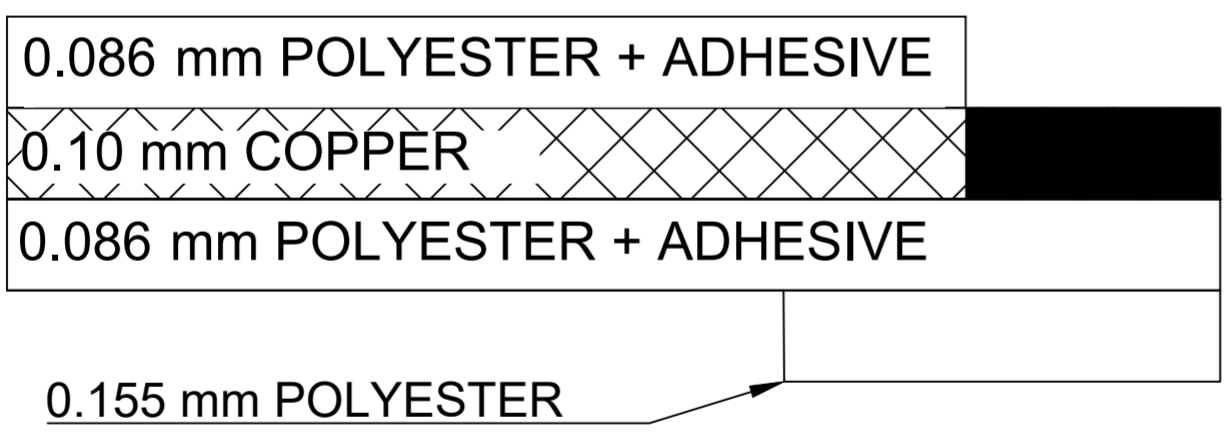
CROSS-SECTION
