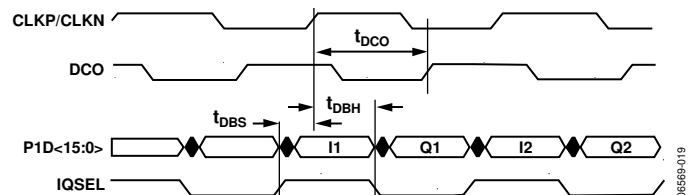
Figure 28. Data Interface Timing, Single-Port Mode
