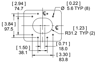
Panel Cutout
