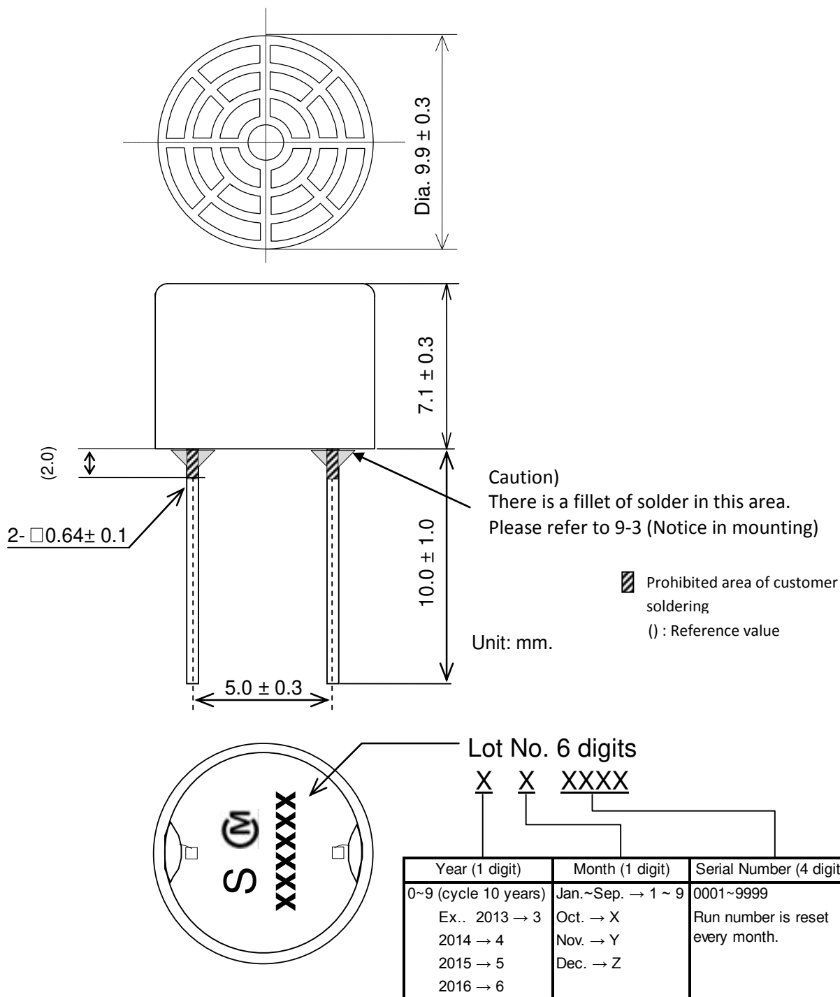
Fig.1: Product Dimension
