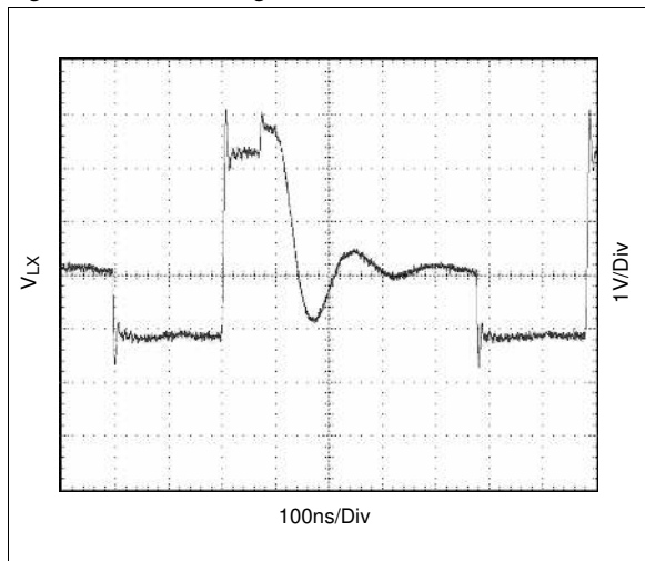
Figure 23. Coil Voltage, I_{OUT} = 1\text{mA}
