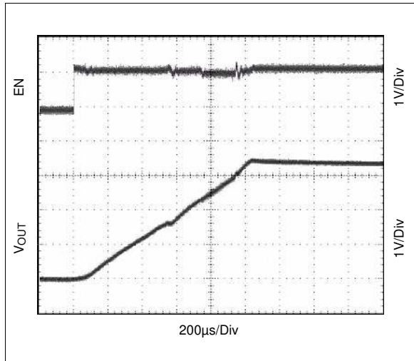
Figure 21. Startup Voltage, I_{OUT} = 1\text{mA}
