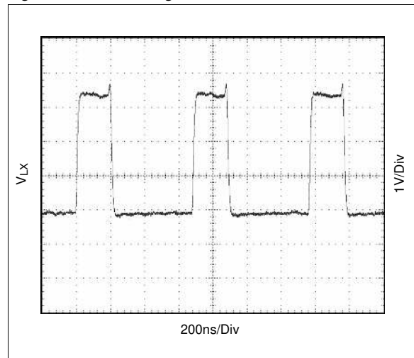
Figure 24. Coil Voltage, I_{OUT} = 100\text{mA}
