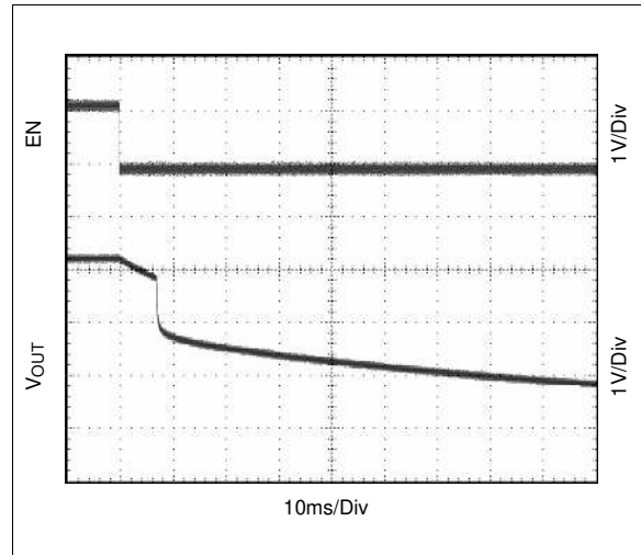
Figure 22. Shutdown Voltage, I_{OUT} = 1\text{mA}
