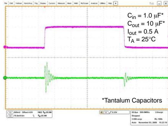
Figure 25. Line Transient Response – V_{out} = 3.3 V
