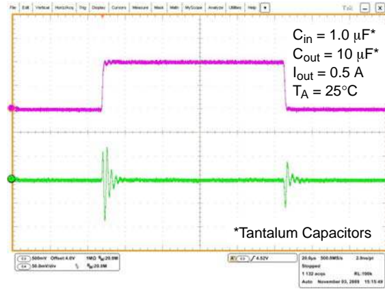
Figure 23. Line Transient Response – V_{out} = 2.5 V
