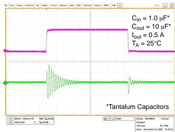
Figure 27. Line Transient Response – V_{out} = 5.0 V
