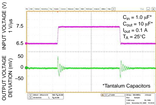
Figure 26. Line Transient Response – V_{out} = 5.0 V
