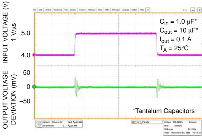
Figure 22. Line Transient Response – V_{out} = 2.5 V
