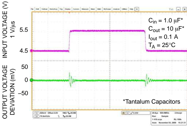
Figure 24. Line Transient Response – V_{out} = 3.3 V
