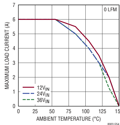
Derating, H-Grade, V_{OUT} = 1.2\text{V} , \text{BIAS} = 5\text{V} , DC2416A Demo Board
