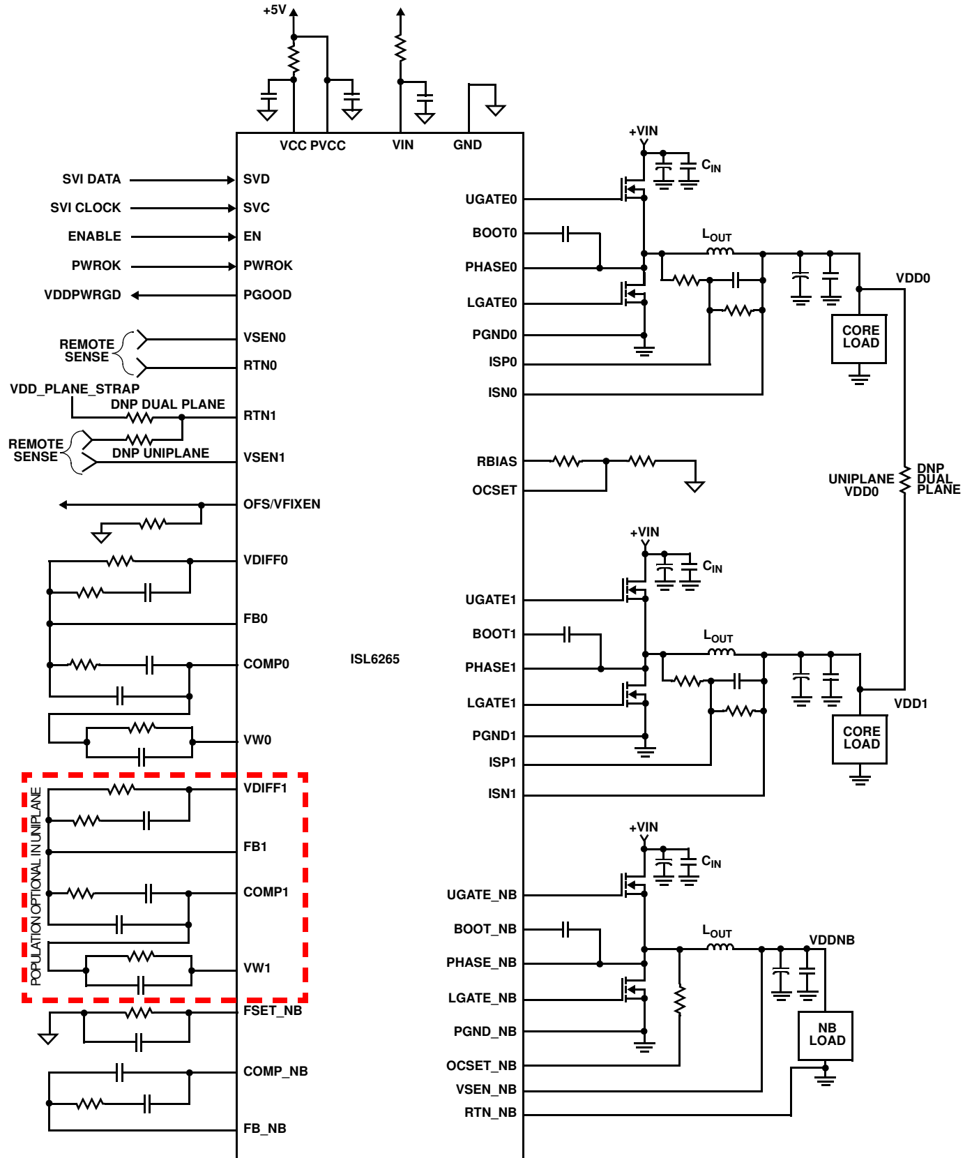
FIGURE 4. ISL6265 BASED UNIPLANE OR DUAL PLANE CORE CONVERTER WITH INDUCTOR DCR CURRENT SENSING
