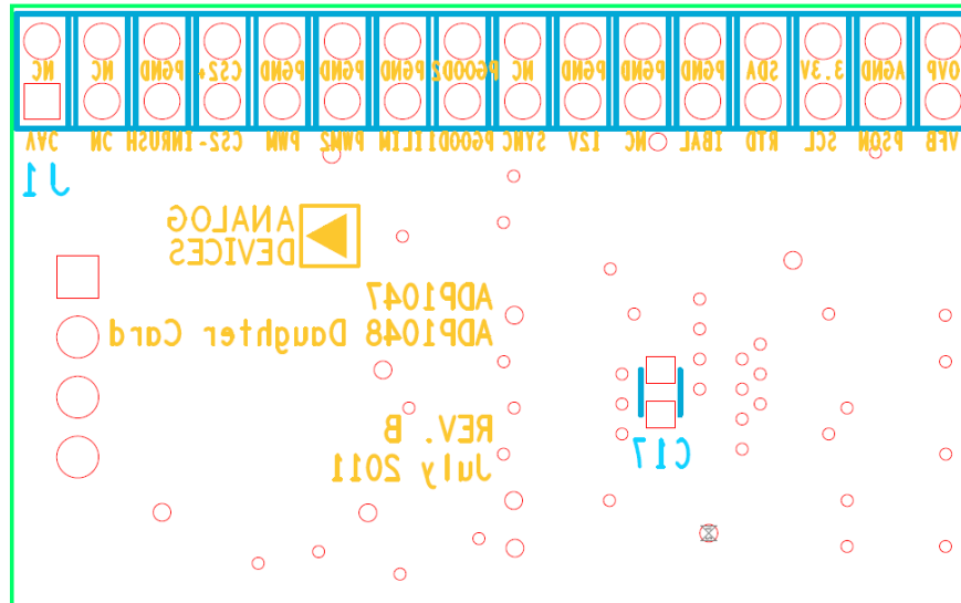
Figure 16 – Bottom Silkscreen
