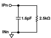
Figure 12. Receiver Simplified Equivalent Circuit When Driving Single-Ended
