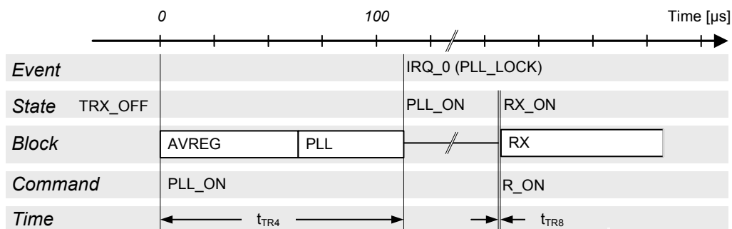
Figure 7-5. Transmission from TRX_OFF to PLL_ON and RX_ON State
