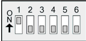
Figure B-08. RS-232 DIP Switch Settings
