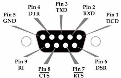
Figure B-09 Pins used on the female RS-232 (DB-9) Serial Connector
