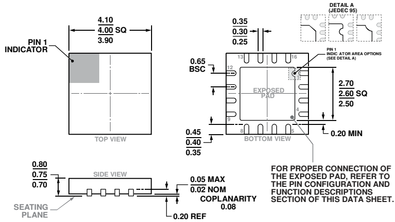
Figure 119. 16-Lead Lead Frame Chip Scale Package [LFCSP] 4 mm × 4 mm Body and 075 mm Package Height (CP-16-17)
