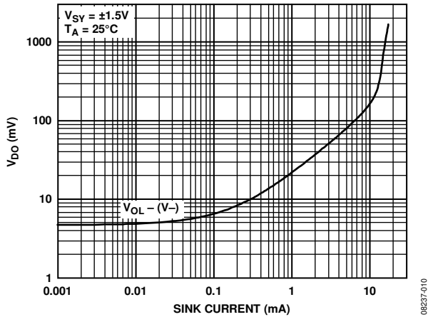
Figure 22. Dropout Voltage ( V_{Do} ) vs. Sink Current
