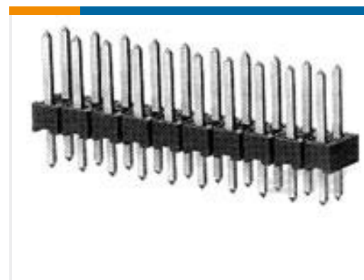
TE Part #5-146258-5 10 MODII HDR DRST B/A .100CL
