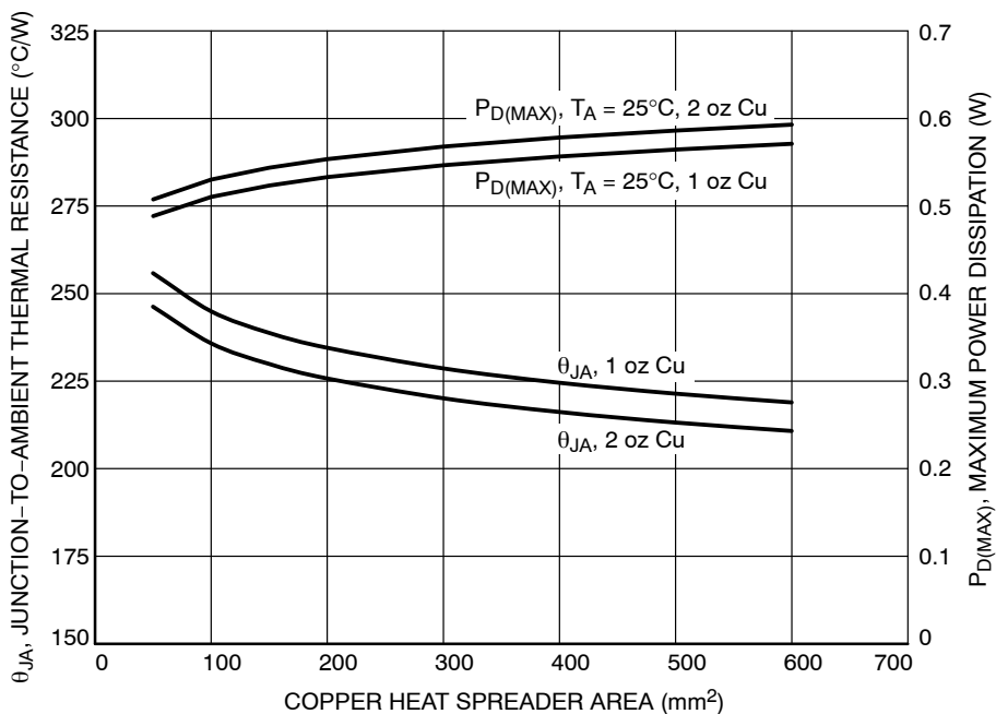
Figure 40. θ JA and P D (MAX) vs. Copper Area (TSOP-5)
