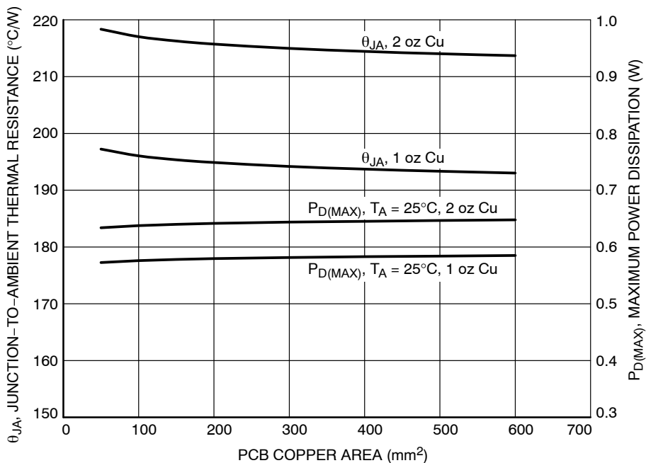
Figure 39. θ JA and P D (MAX) vs. Copper Area (XDFN4)
