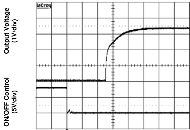
Figure 4. Start-Up from Enable Control (typical Vin, zero load)
