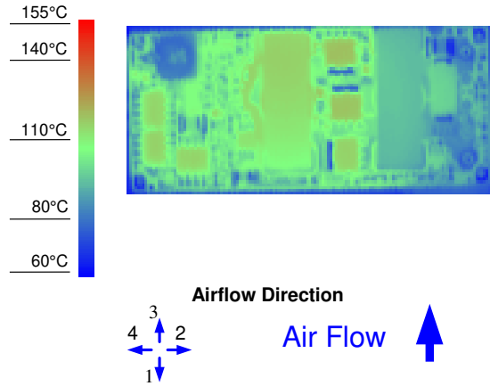
Figure 8. Thermal Image for Airflow Direction 3 (30A output, 55°C ambient, 200 LFM, typical Vin, open frame, socket interface)
