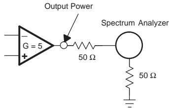
TEST CIRCUIT FOR IMD 3 / OIP 3
