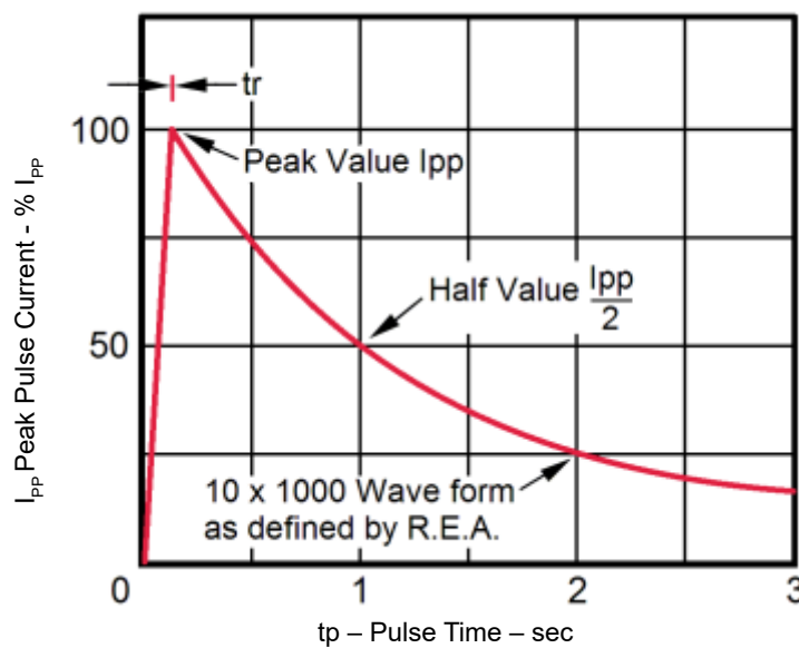
Figure 2 Pulse Waveform Test waveform parameters: t_r = 10 \mu\text{s} , t_p = 1000 \mu\text{s}
