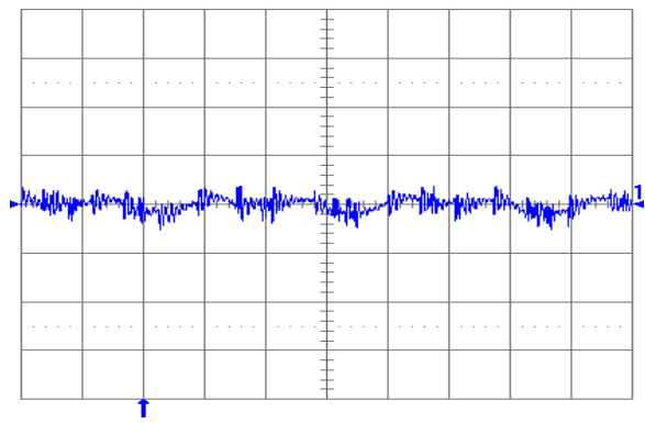
Fig. 1.0V.6: Output voltage ripple (20 mV/div.) at full rated load current into a resistive load with external capacitance 47\ \mu\text{F} ceramic + 1\ \mu\text{F} ceramic, and V_{in} = 5\text{ V} for V_{out} = 1.0\text{ V} . Time scale: 2 \mu\text{s} /div.
