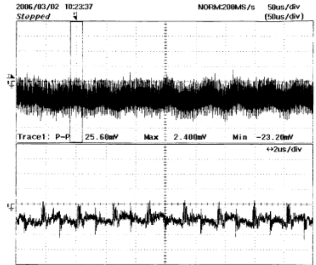
Figure 25 – Ripple, 48 VDC, Full Load. Upper: 50 \mu s / div, 10 mV / div. Lower: 2 \mu s / div, 10 mV / div.
