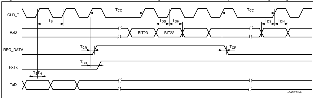
Figure 9. Data transmission -> control reg. write -> data reception timing diagram
