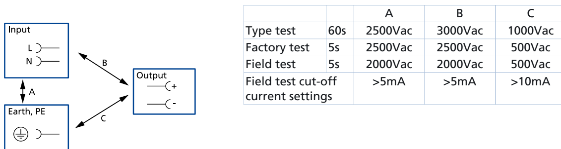
Fig. 17-1: Dielectric strength
