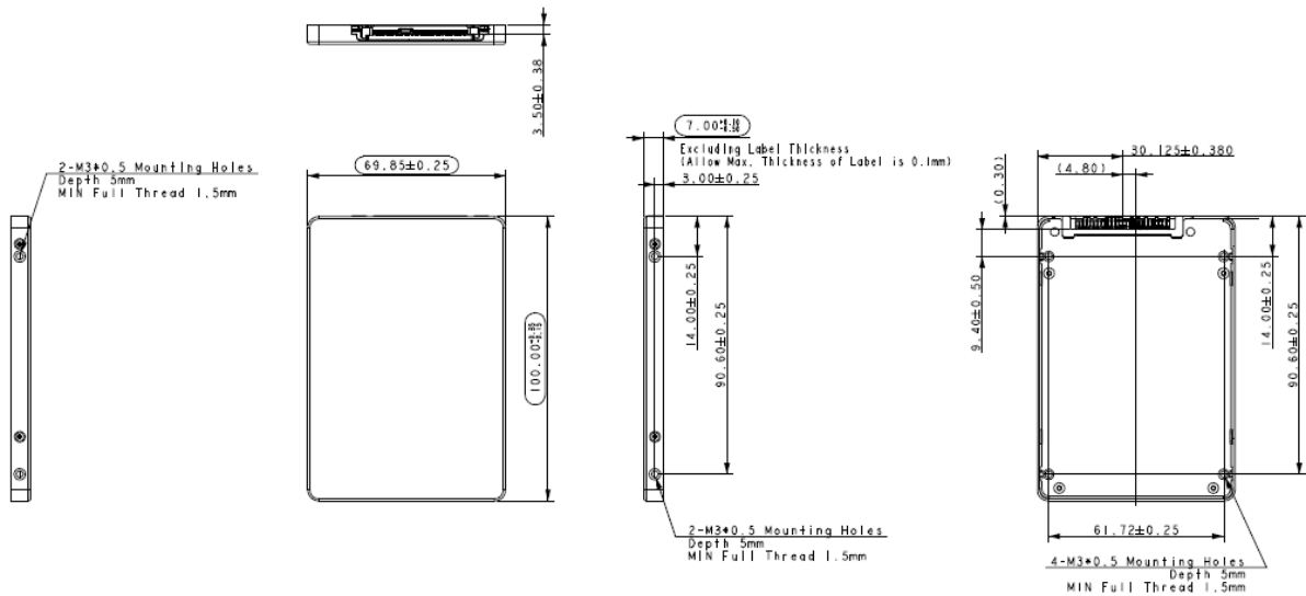
Figure 9-1 Physical Dimensions
